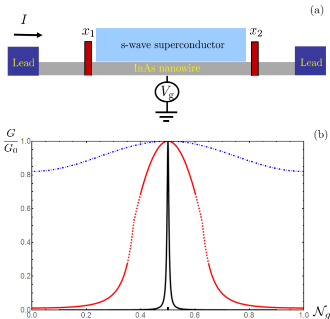
FIG. 1. (Color online) Panel (a): Schematic plot of the device. Panel (b): Conductance G as a function of the dimensionless gate voltage N_g . In a symmetric device, g_1 = g_2 \equiv g , conductance reaches G_0 . Solid (black) curve: Coulomb blockade peak at g \ll 1 is a Lorentzian [33] of width given by Eq. (25). Dashed/solid (red) curve: G(N_g) at intermediate values of g such that \Delta_P/E_C \ll 1 - g \ll 1 ; see Eq. (23) for the width of the maximum and Eq. (24) for the crossover to the weak-tunneling limit. Dot-dashed (blue) curve: G(N_g) of a symmetric device in the strong-tunneling limit, E_C(1 - g) \ll \Delta_P . Conductance approaches the unitary limit, exhibiting weak N_g -dependent oscillations, see Eq. (22).
